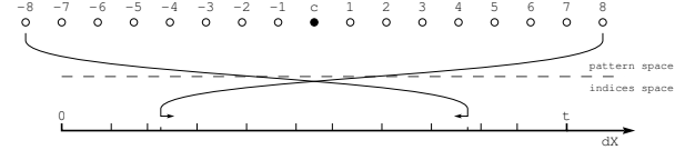
Figure 6: Inspecting the immediate neighbor location outside the window of Figure 5 reveals two dual-context IDs.
