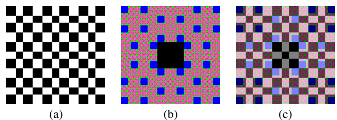
Figure 11: Set-region maps of AA(\sqrt{3}) : (a) The neighborhood map from Figure 7. (b) The coloring map for Figure 3(b). (c) The superposition of the two maps: the neighborhood map tends to align with the blue blocks because our chosen neighborhood window is the same order of size as the blue clusters in Figure 3(a).
