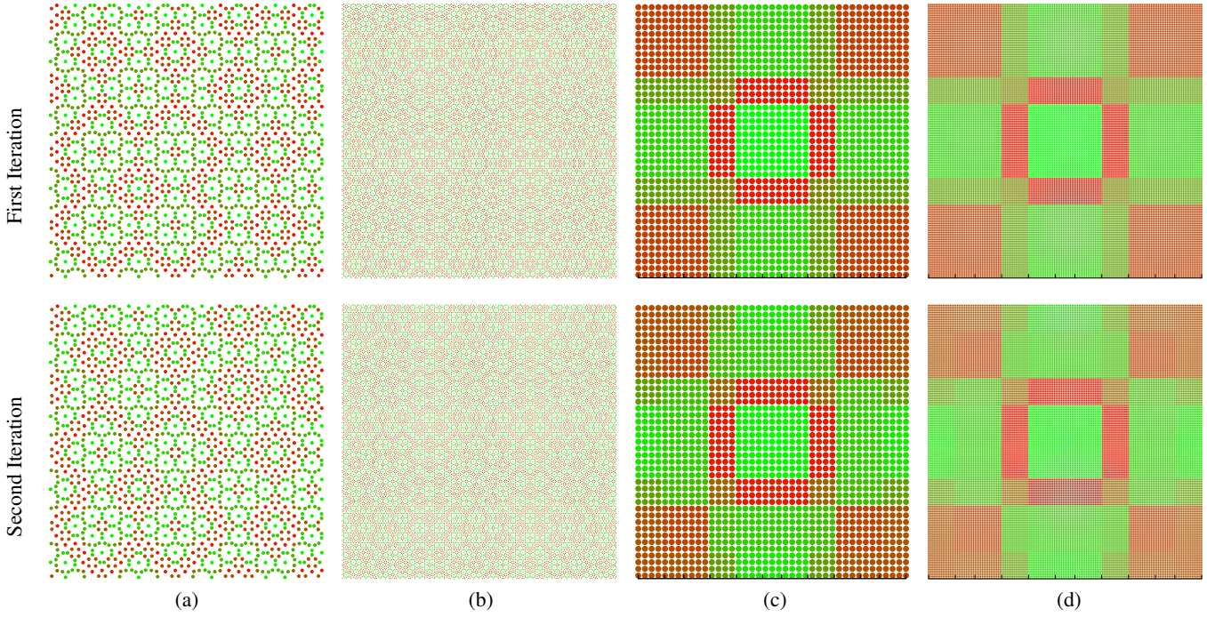
Figure 9: Visualization of two iterations of Lloyd’s algorithm applied to a single period of AA(97/56) and AA(362/209) , where 97/56 \approx 362/209 \approx \sqrt{3} . (a, b), respectively, show the actual displaced point set, where each point is colored according to the size of incurred displacement; in a smooth scale from green (0) to red (largest displacement). In (c, d), respectively, we rearranged the points by order of their indices; in other words, we plotted the sizes of displacements in index-space. For comparison, the ticks below each index-space plot show the thresholds of Figure 5 at the right scale.
