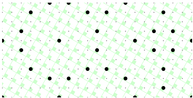
Figure 2: An AA Pattern is obtained when an appropriately transformed array of cells is used to filter points in the integer grid. A point is retained iff it hits the set (green) region of a cell.
