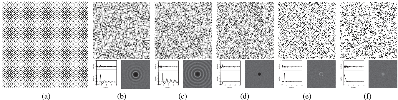
Figure 1: (a) AA(183/112); converted into (b) BNOT blue noise profile [de Goes et al. 2012], (c) FPO-like profile ( \delta_{min} = 0.925 ) [Schlömer et al. 2011], (d) step blue noise [Heck et al. 2013], (e) green noise (using [Heck et al. 2013]), and (f) pink noise (using [Heck et al. 2013]).
