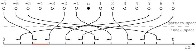
Figure 5: In a row of the dX -bitmap of AA(\sqrt{3}) , examining a window of width 15 generates 10 thresholds that partition the indices into 11 intervals, corresponding to 11 distinct pattern-space layouts of neighbor points. We make it clear that ‘15’ is an arbitrarily chosen width, and does not have a special meaning; any other width gives analogous results.
