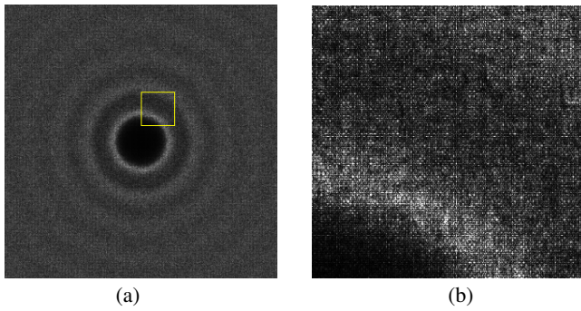
Figure 10: (a) Power spectrum of a 64k blue-noise point-set generated with Algorithm 3 using a 5k table. (b) A closeup showing the quantized nature of the spectrum.
