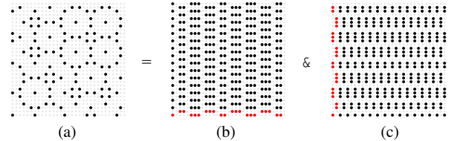
Figure 4: (a) A part of AA(\sqrt{3}) , and its constituent (b) dX -bitmap and (c) dY -bitmap; highlighting the constituent pair of (b) rows and (c) columns.
